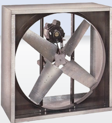
Industrial Grade Exhaust Fan (Requires 53" x 53" Framed Opening)
